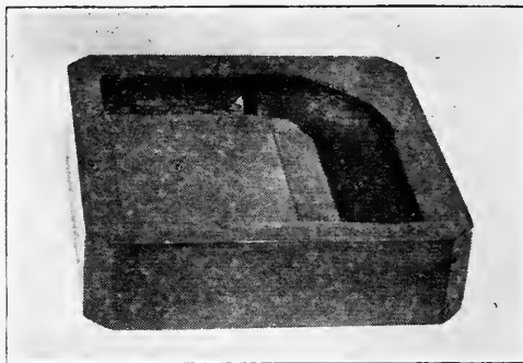
FIG. 538. ONE-PART CORE-BOX.
